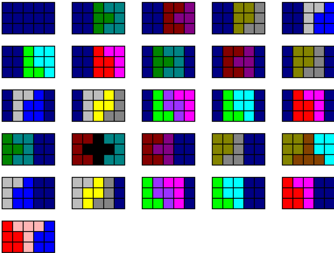
Figure 2: The 26 solutions for N = 5
