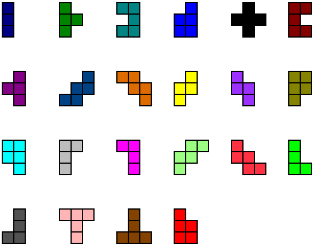
Figure 1: The 22 allowed pieces of the puzzle.
