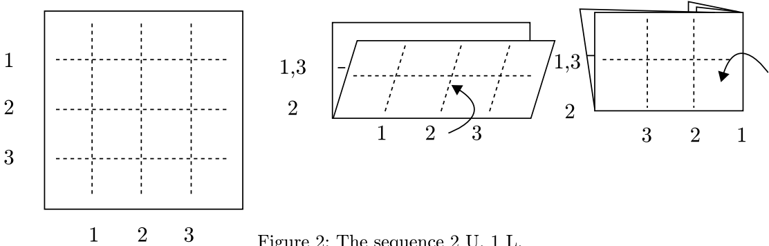
Figure 2: The sequence 2 U, 1 L.
